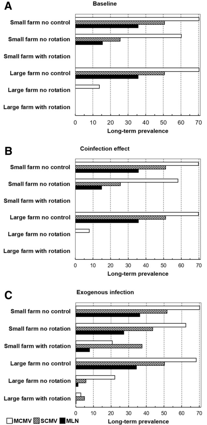
Fig. 6. Long-term Maize chlorotic mottle virus (MCMV), Sugarcane mosaic virus (SCMV), and maize lethal necrosis (MLN) prevalence for different management strategies and epidemiological scenarios, showing long-term prevalence of each virus when there is disease management, as well as the long-term prevalence of MLN. A , Baseline parameterization; B , coinfecting seed causes increased vertical transmission; and C , exogenous infection. Note that, in A and B, the two “No Control” scenarios again lead to identical results whereas, in C, there is a slight difference between the results of these scenarios.
